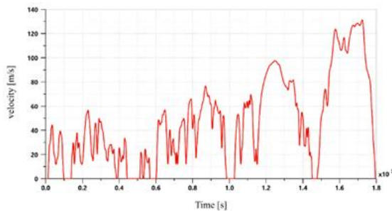
Figure 2: WLTC
